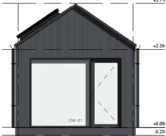
FACADE ON AXIS B-A M 1 : 50
